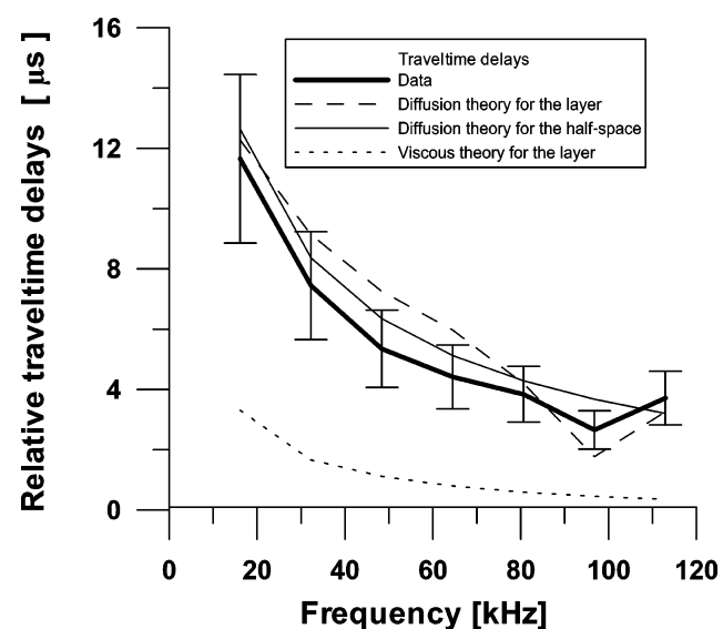
Figure 6. Traveltimes delays of a reflected wave from a dry layer with respect to a water-saturated layer. Data curve (thick solid line) is compared with the theoretical diffusive-viscous model (dashed line) and purely viscous model (dotted line). A theoretical curve for a diffusive-viscous half-space is shown as thin solid line.
