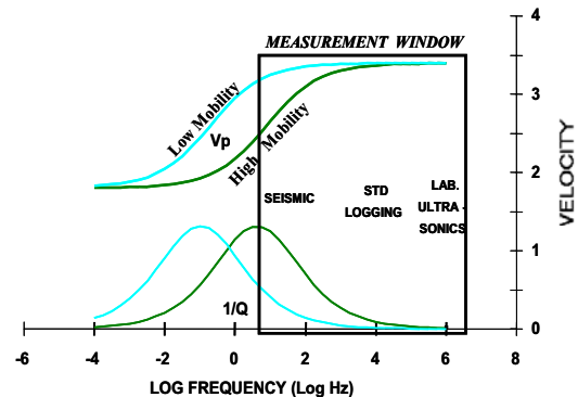
Figure 1. Cole-Cole relation couples velocity and attenuation as functions of frequency. The frequency range of our laboratory measurements is indicated. Also shown is the effect of high fluid mobility and low fluid mobility.
